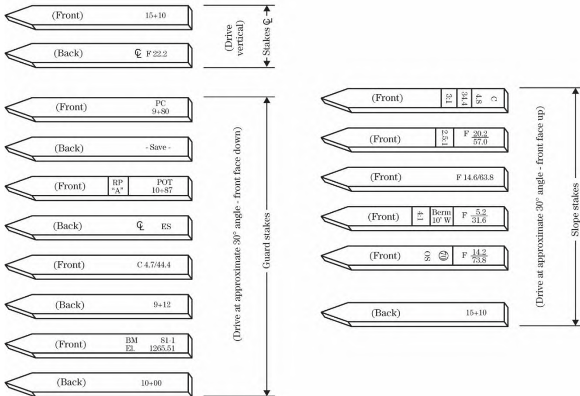
Figure 1-72: Slope Stakes
