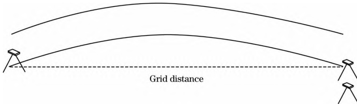
Figure 1-83: Relationship of the Ground Distance to the Grid Distance. Because the Grid is Planar, it can be Simply Stated That the Lengths on the Grid Surface are Shorter Than Lengths on the Ground Surface.
