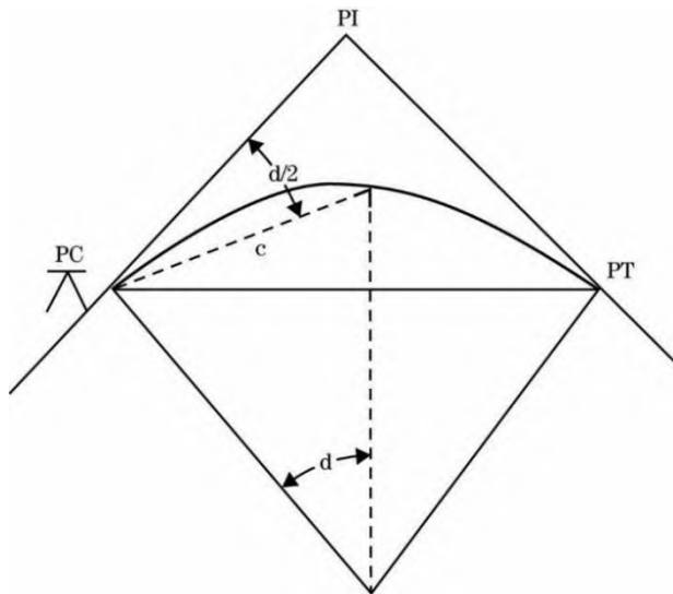
Figure 1-99: Principle of Curve Layout by Deflection Angle
