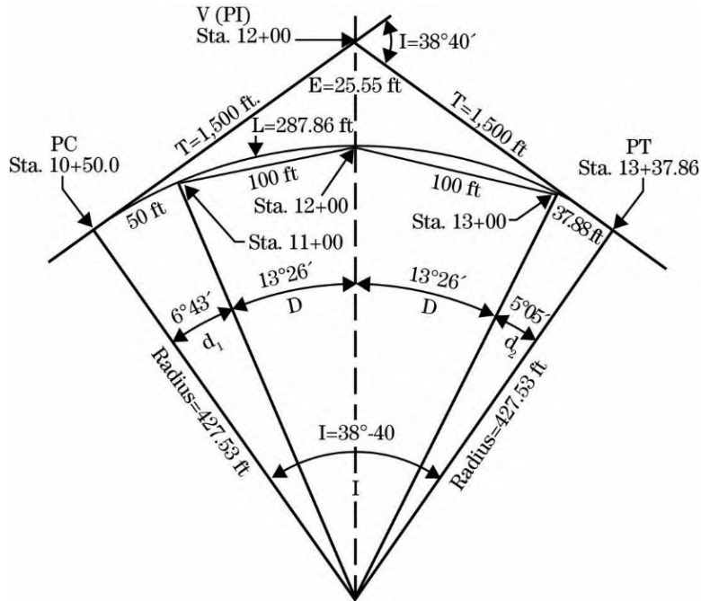
Figure 1-98: Elements of a Circular Curve
