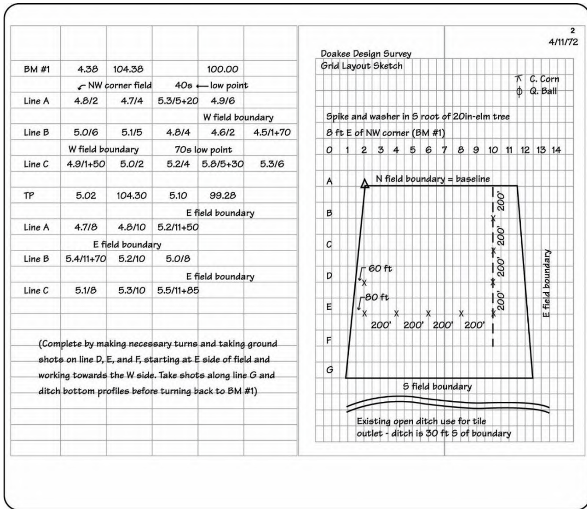
Figure 1-65: Survey Notes—Grid Survey
