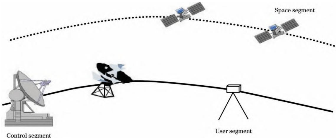
Figure 1-73: Conceptual Diagram of the Three Major Segments that Comprise the GPS
