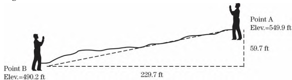
Figure 1-28: Calculation of Vertical Distance
