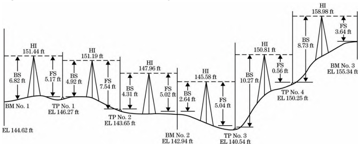
Figure 1-66: Method of Differential Leveling
