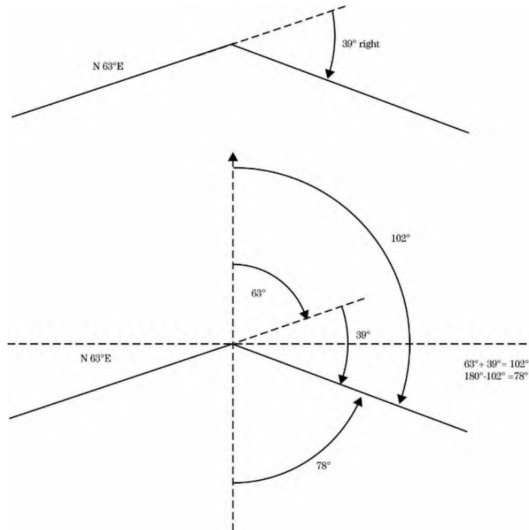
Figure 1-26: Course Direction Determination from Measured Angles
