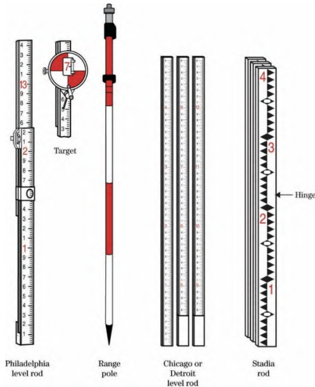
Figure 1-41: Types of Level Rods and Range Pole
