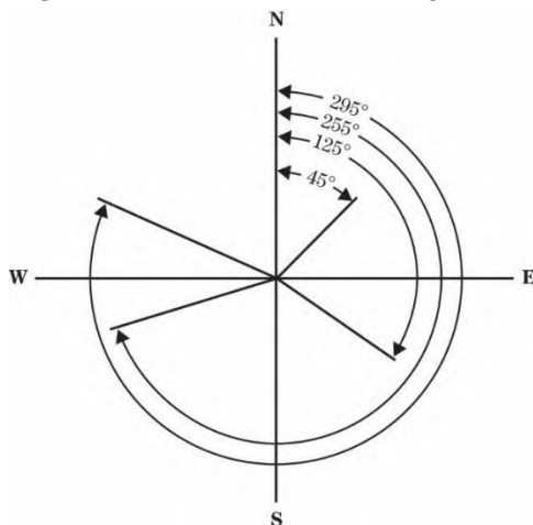
Figure 1-61: Azimuths Showing 0^\circ Oriented to the North
