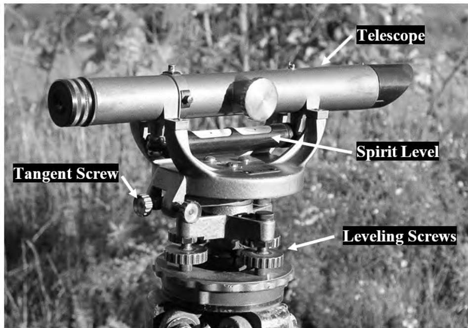
Figure 1-39: Dumpy Level
