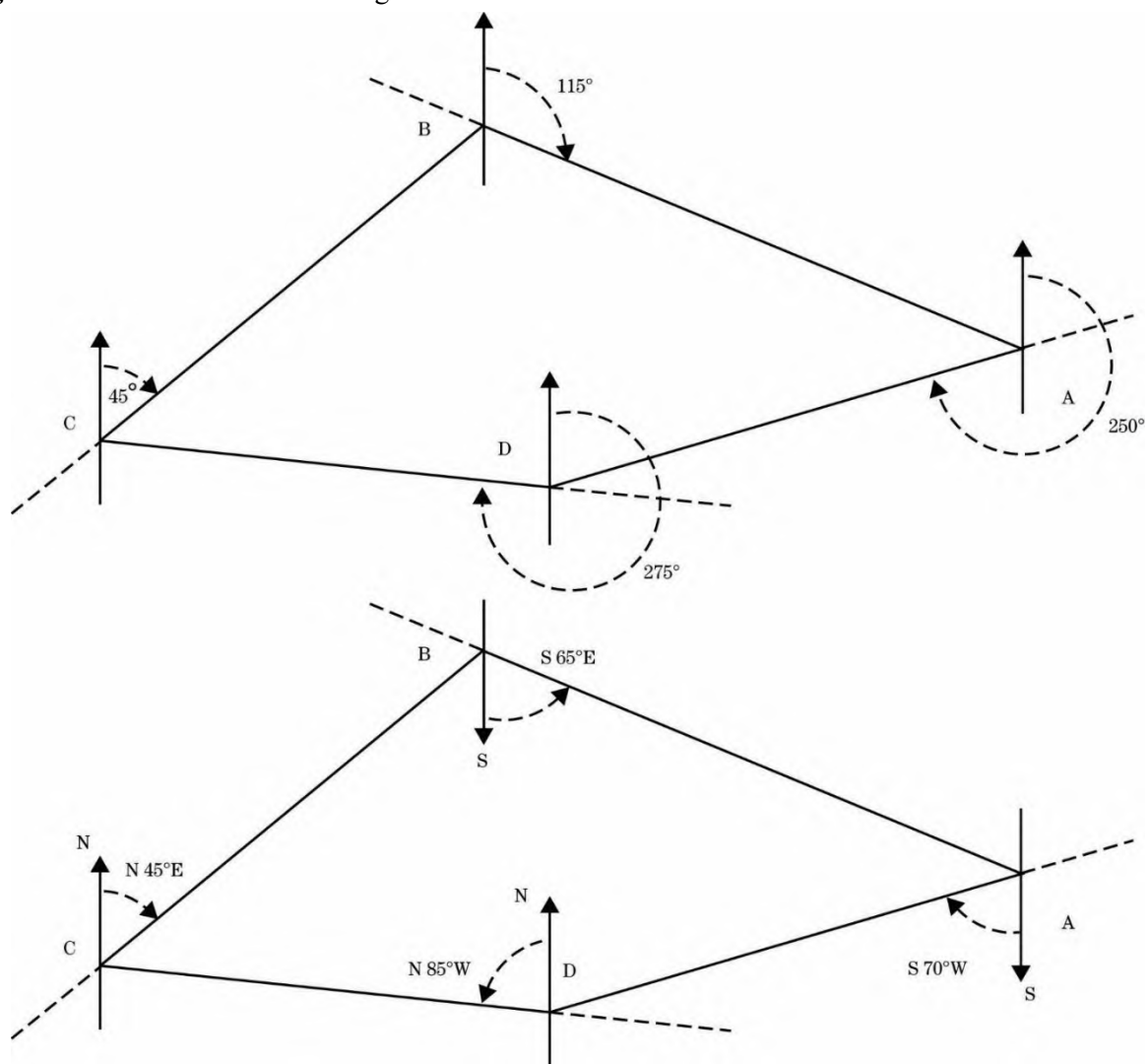
Figure 1-15: Azimuths and Bearings
