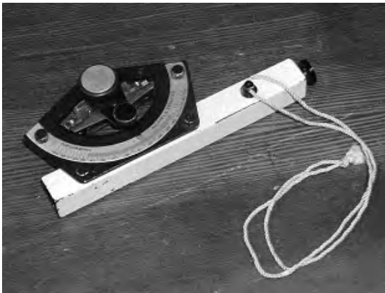
Figure 1-43: Abney Hand Level
