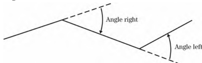
Figure 1-25: Deflection ANGLES as Extensions of the Previous Course
