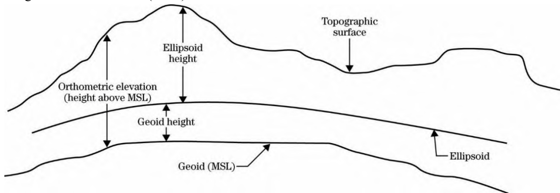
Figure 1-82: The Relationship of the Geoid Model, Ellipsoid Model, and Topographic Ground Surface to Each Other. In Typical Profile Leveling, the Topographic Surface or Orthometric Height Above the Geoid (MSL) Is Derived.
