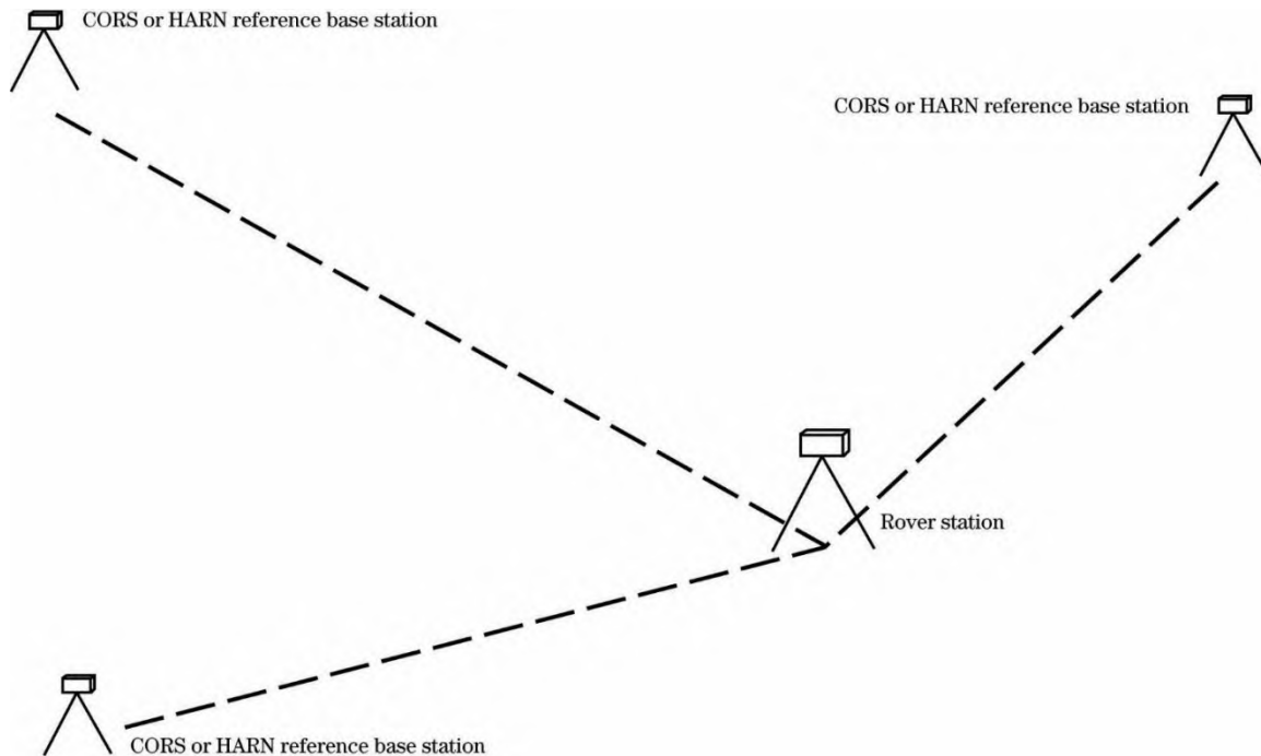
Figure 1-75: Conceptual Diagram of a Large Area Reference Base Utilizing Multiple Available CORS or the High Accuracy Network Service, HARN Network Reference Base Positions
