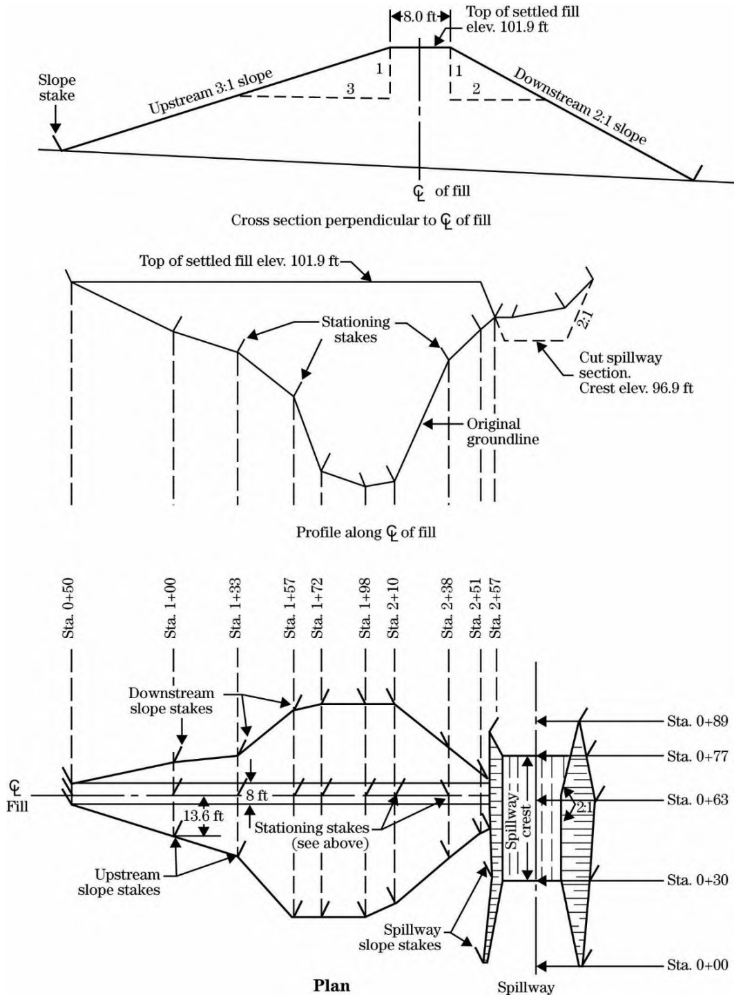
Figure 1-70: Grade Rod Method for an Earth Dam
