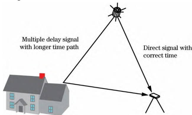
Figure 1-78: Multipath Delay is Caused by the Deflection of the Incoming GPS Signal off of a Reflective Object Prior to Hitting The Receiver Resulting in a Longer Time Path
