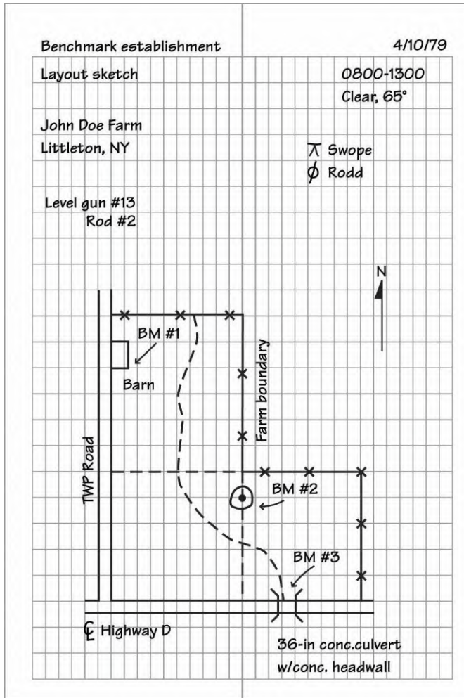
Figure 1-67: Survey Notes for a Bench Level Circuit
