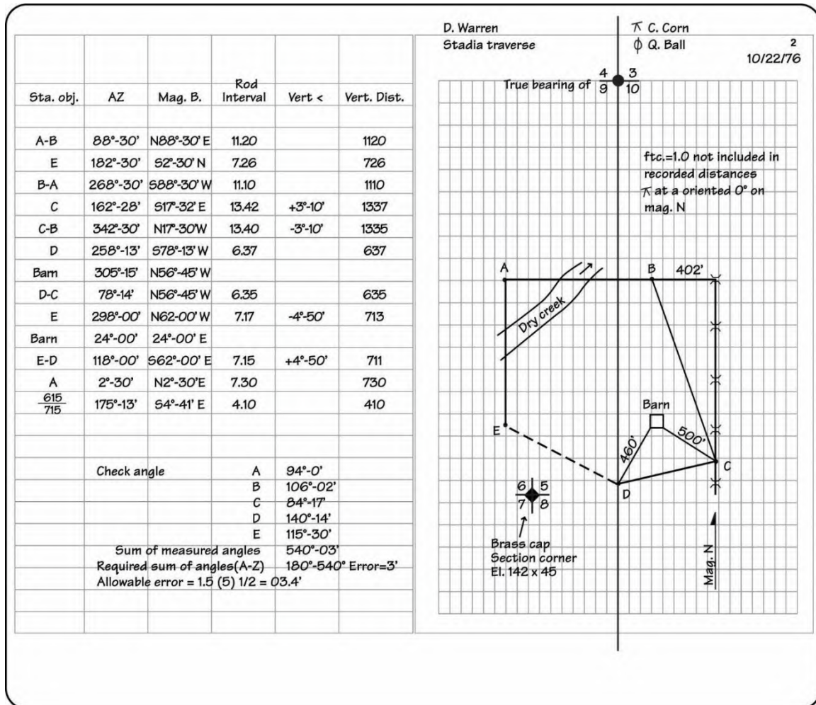
Figure 1-62: Survey Notes—Stadia Traverse Survey for Horizontal Control (English)
