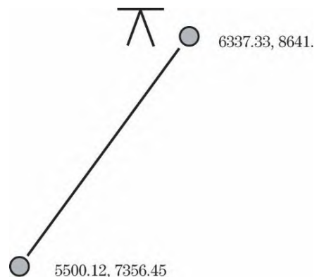
Figure 1-55: Backsight from the Instrument Position at Point 2
