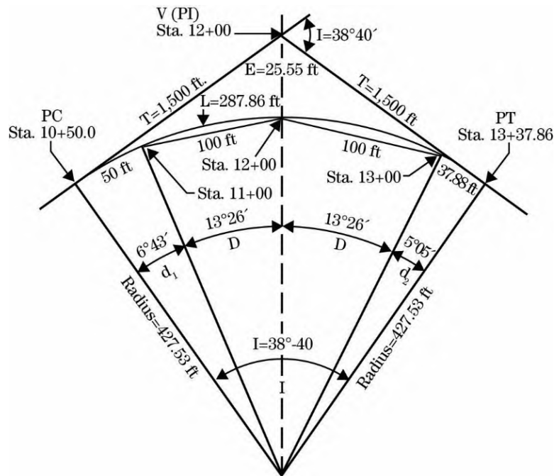
Figure 1-100: Layout of Circular Curve (English)
