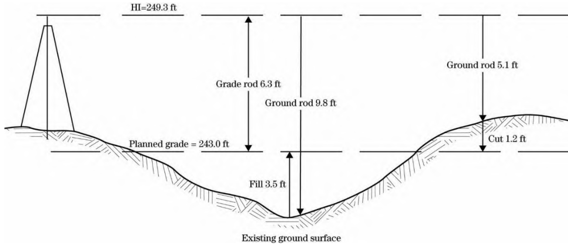
Figure 1-69: Survey Notes—Ditch Survey Using the Grade Rod
