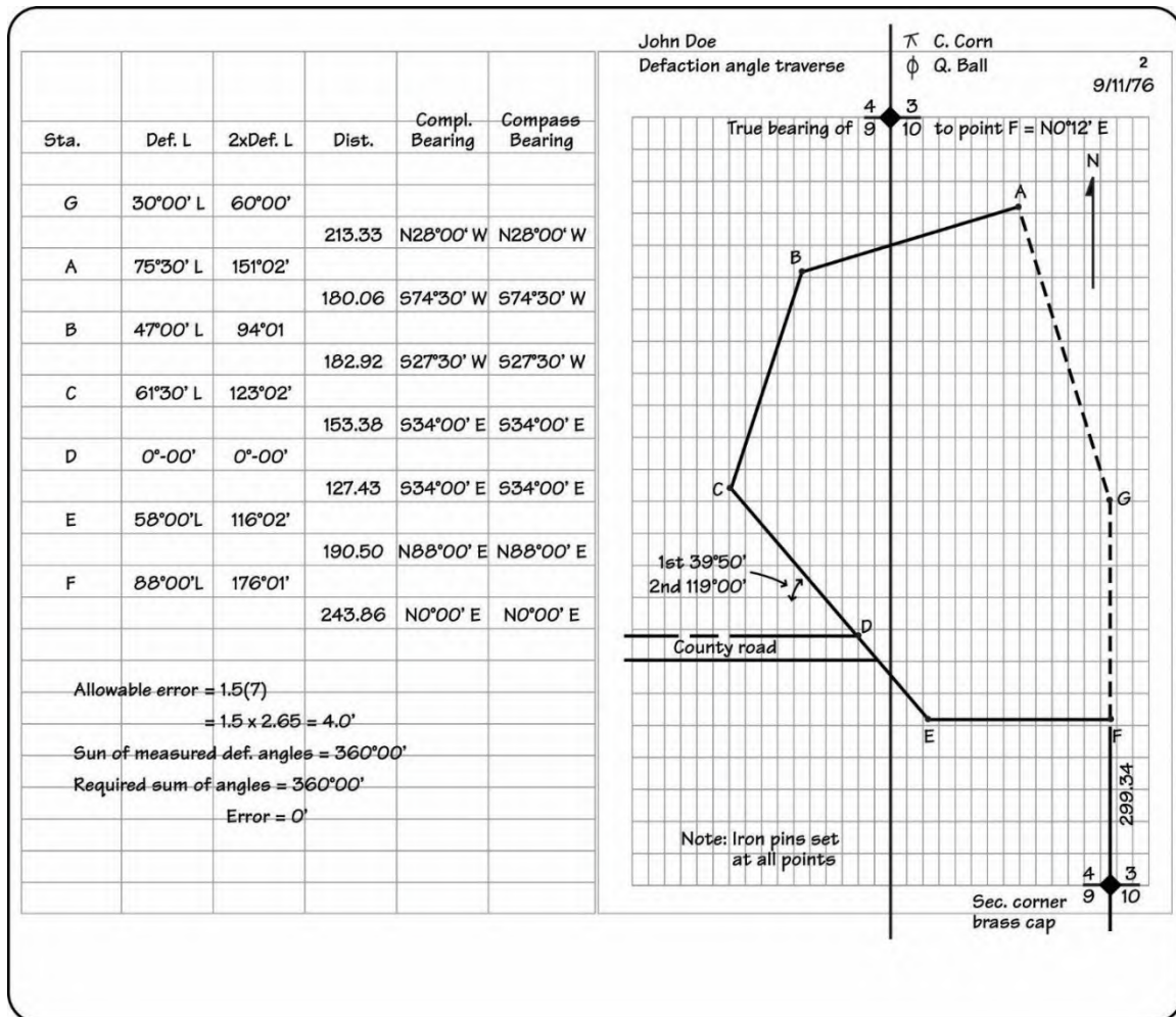
Figure 1-60: Survey Notes for the Deflection Angle Example
