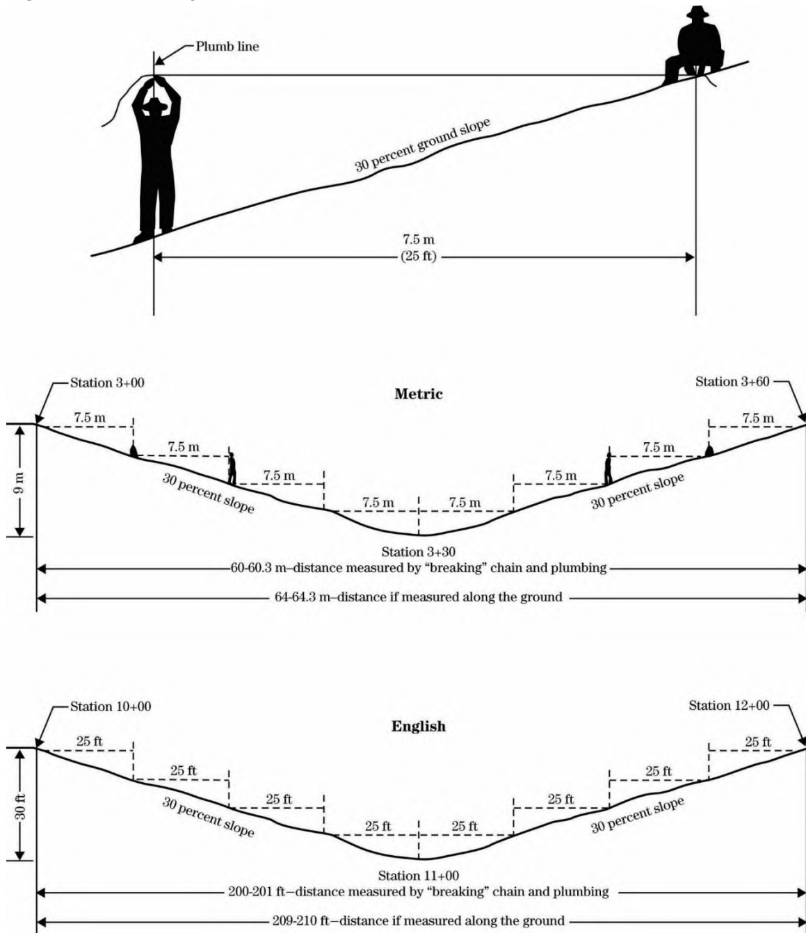
Figure 1-21: Breaking Chain
