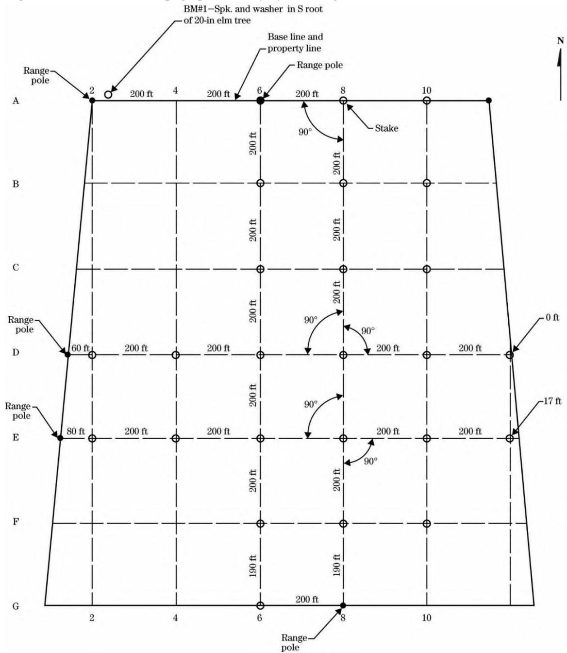
Figure 1-64: Method of Topographic Survey by Gridding
