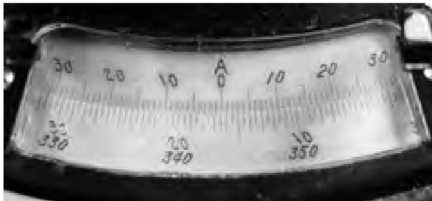
Figure 1-57: One-minute Vernier Set for Measurement
