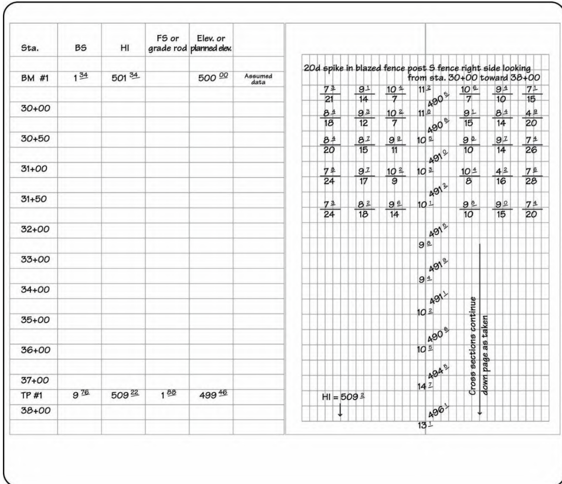
Figure 1-68: Survey Notes—Profile and Cross Section - continued
