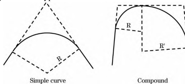
Figure 1-95: Types of Route Curves
