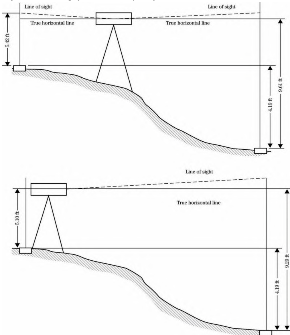
Figure 1-52: Two-peg Method for Adjusting Levels
