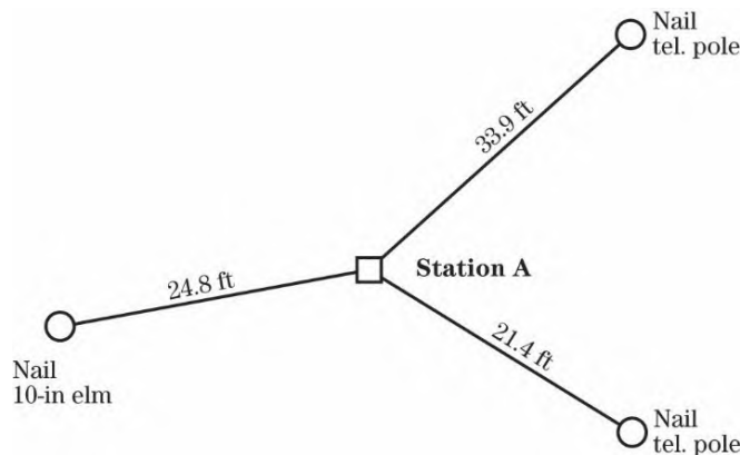
Figure 1-58: Offset Ties to a Traverse Station
