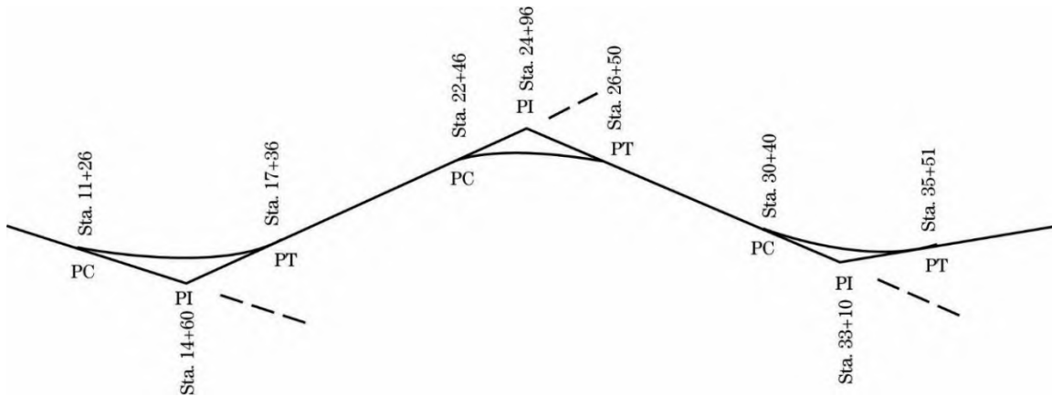
Figure 1-956: Circular Curves in a Traverse Survey
