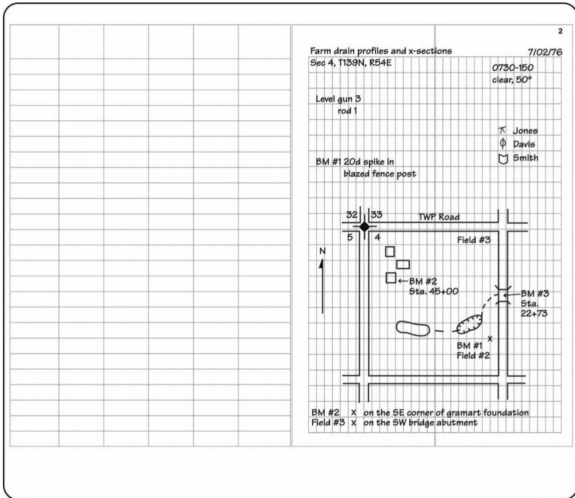
Figure 1-68: Survey Notes—Profile and Cross Section
