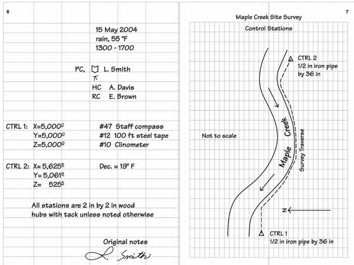
Figure 1-3: Set of Field Survey Notes - continued
