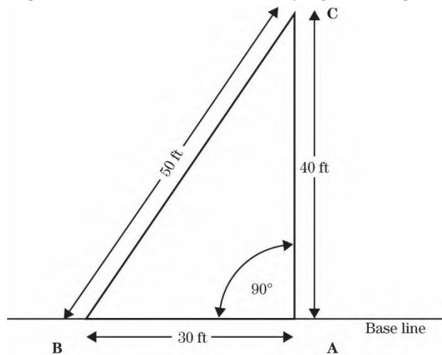
Figure 1-63: 3-4-5 Method of Laying out a Right Angle
