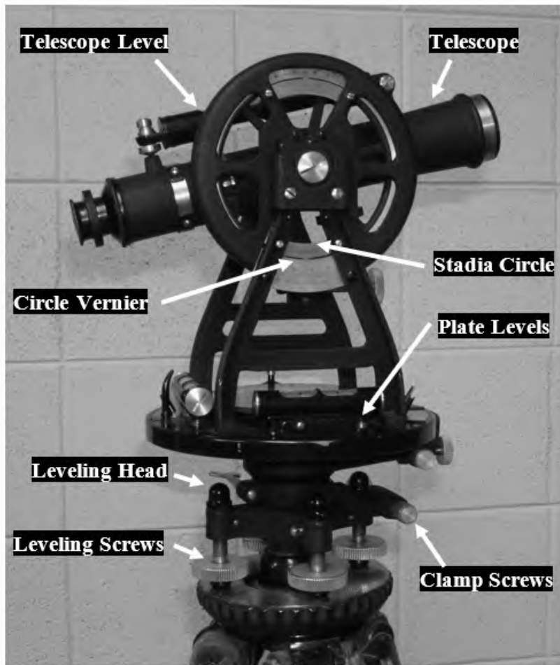
Figure 1-46: Engineer's Transit
