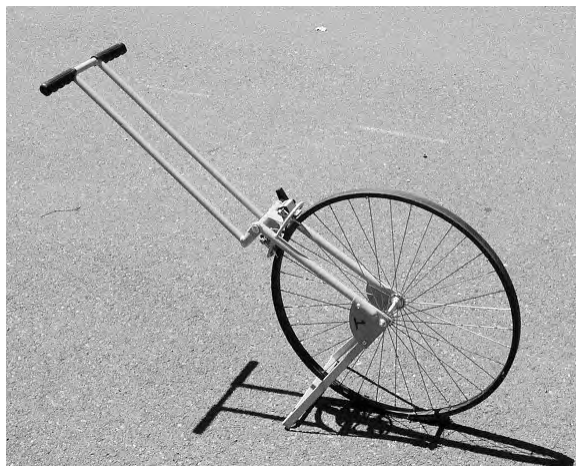
Figure 1-20: Odometer Wheel
