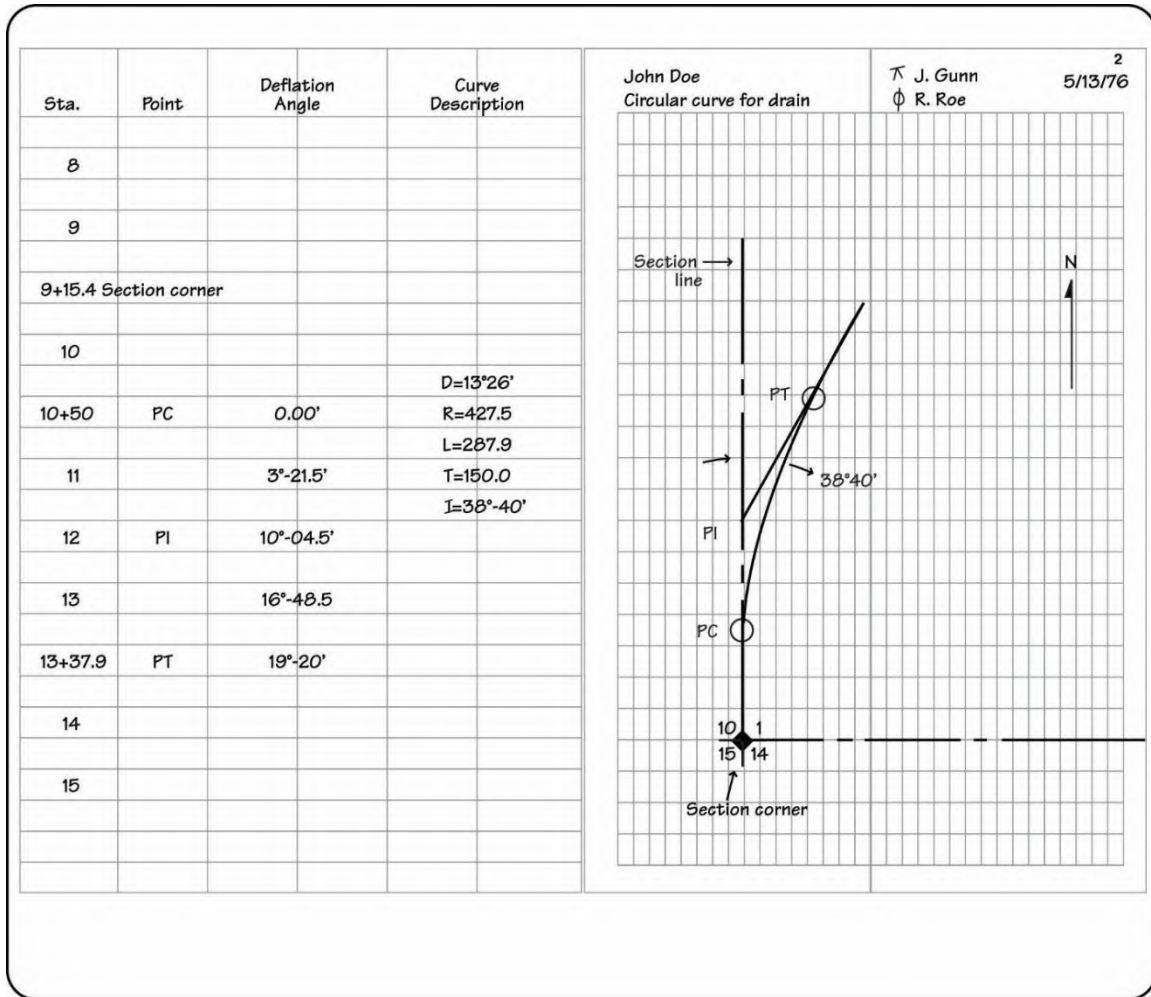
Figure 1-101: Survey Notes--Circular Curve - continued
