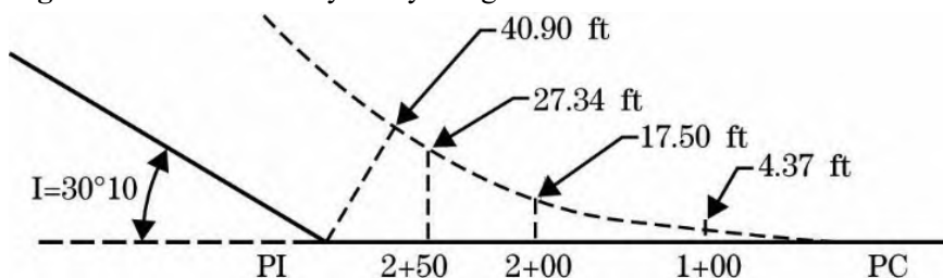
Figure 1-102: Curve Layout by Tangent Offsets
