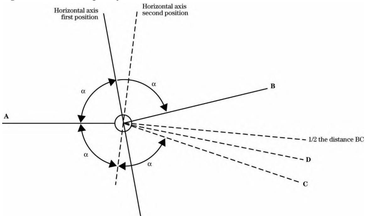
Figure 1-53: Line of Sight Adjustment for the Transit and Theodolite
