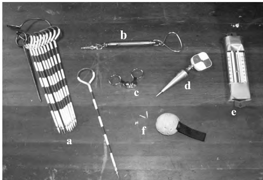
a. Chaining pins, b. Chain tensioner, c. Tape clamps, d. Plumb bob with gammon reel, e. Thermometer, f. Tack ball
