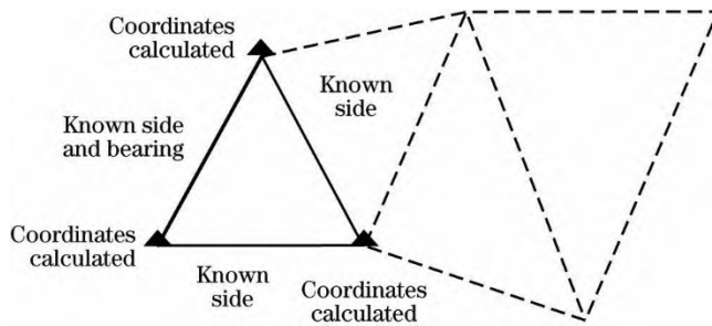
Figure 1-14: Control Survey (Trilateration)
