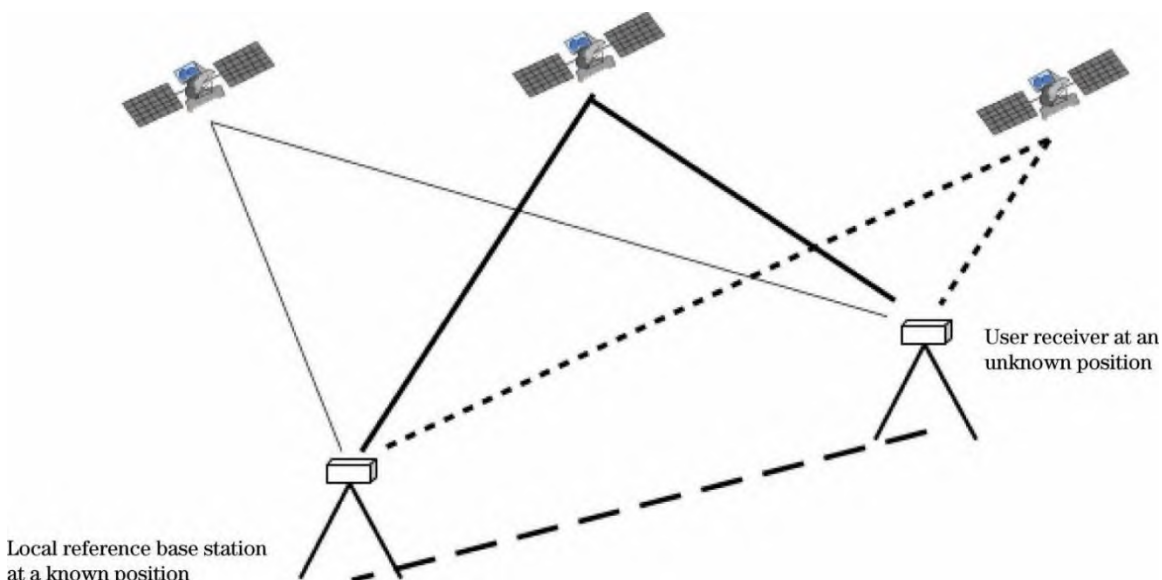
Figure 1-74: Conceptual Diagram of the Differential Baseline Setup to an Unknown (Rover) Position. Note that Both Positions are Receiving the Same Satellite Signals.
