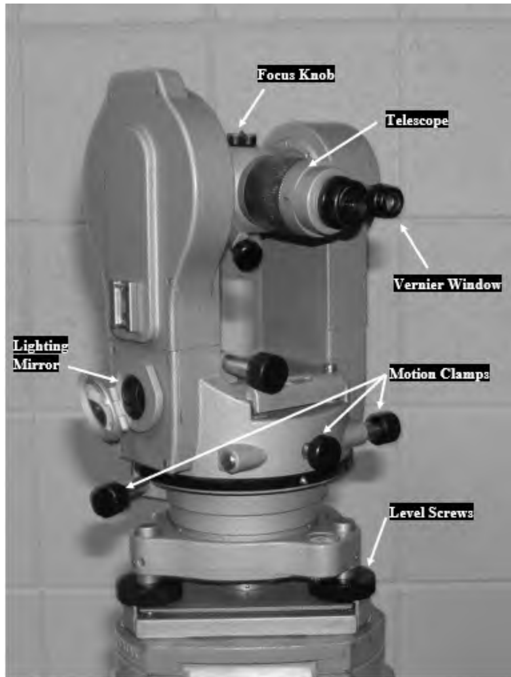
Figure 1-47: Electronic Theodolite
