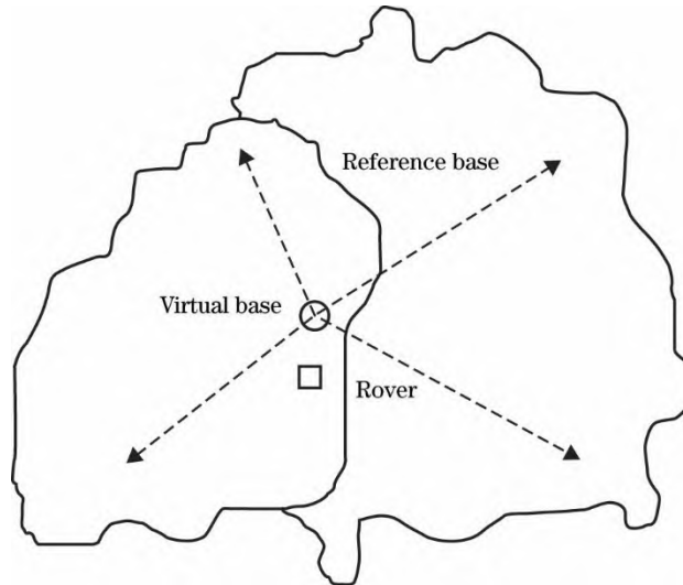
Figure 1-85: Conceptual Setup for eRTK using Virtual Reference Technology. The VRS Generate a Virtual Reference Position in the Vicinity of the Rover and Transmit this via a Cellular Phone Network. Area Coverage Expands the Traditional RTK by Magnitudes.
