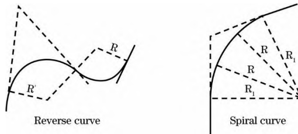
Figure 1-95: Types of Route Curves - continued
